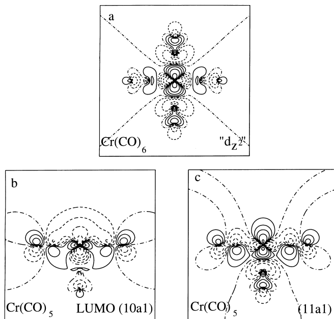
Fig. 3. (a) Orbital contour plot of the virtual e_g^* ("d z 2 ") orbital of \text{Cr(CO)}_6 . Contour values: \pm 0.5 , \pm 0.2 , \pm 0.1 , \pm 0.05 , \pm 0.02 and 0.0 ( e \text{ bohr}^{-1} ) 1/2 . (b) Orbital contour plot of the a_1 LUMO of \text{Cr(CO)}_5 , which is similar to the 10a_1 SOMO of \text{Mn(CO)}_5 . (c) Orbital contour plot of the 11a_1 \sigma' orbital of \text{Cr(CO)}_5 (similar to 11a_1 of \text{Mn(CO)}_5 ).
