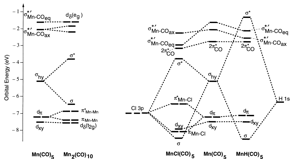
Fig. 4. Orbital interaction diagram for the formation of \text{Mn}(\text{CO})_5\text{L} , where \text{L} = \text{Mn}(\text{CO})_5 , \text{Cl} or \text{H} . The \text{Cl } 3\text{p} level is not at the energy calculated in the neutral atom but is positioned so as to suggest correctly the composition of the orbitals.
